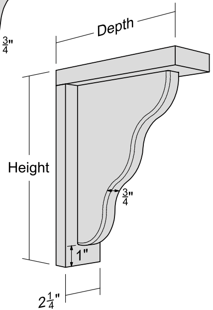
3B 3 Bump Corbel with Backer Board
