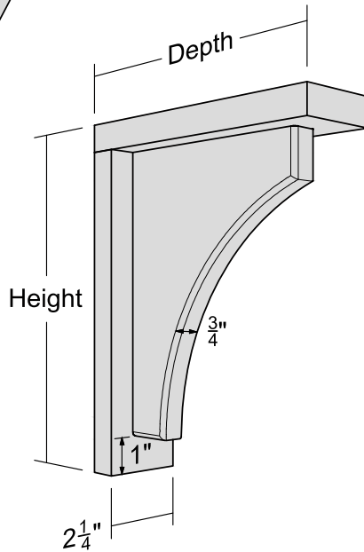
C Curved Corbel with Backer Board
