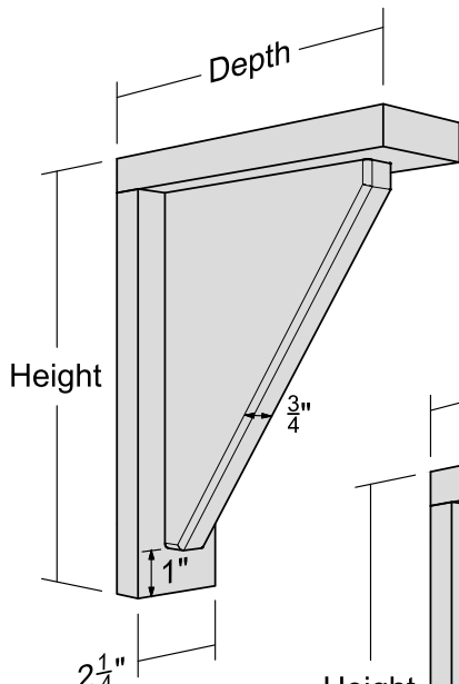
A Angled Corbel with Backer Board
