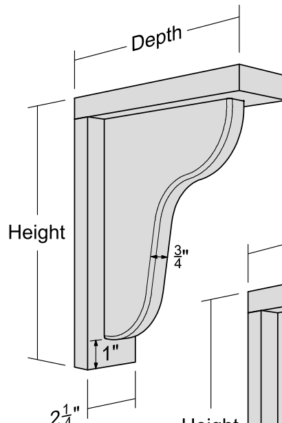
2B 2 Bump Corbel with Backer Board
