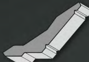
Crown - J1612 78.8(3 1/8") x 54.4(2 1/8")
